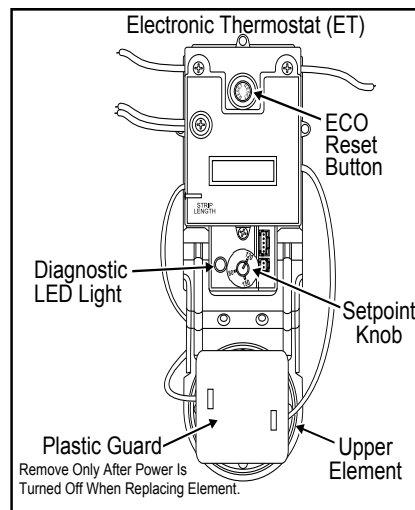
Figure 21 - Electronic Thermostat
