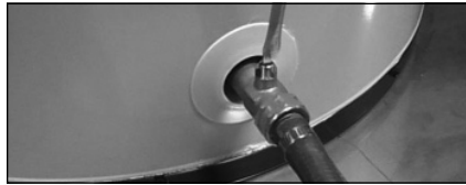
Figure 38 - Drain Valve
