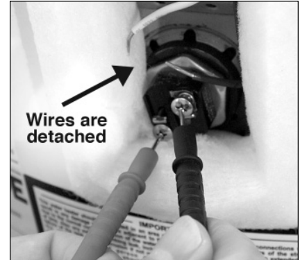
Figure 25 - Use a multimeter to check the resistance of the upper heating element.
