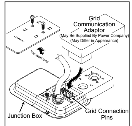
Figure 23 - Smart Grid Connection
